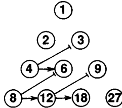
Figure 12. The harmonic proportions with the three harmonic means of 4, 8 and 12.
